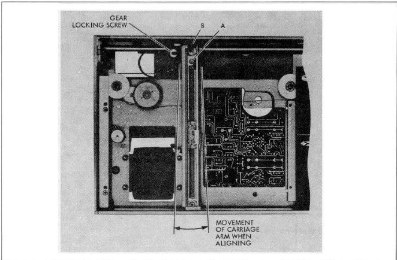
FIGURE 5-19. Y-AXIS ALIGNMENT
