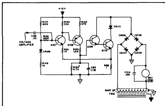
FIGURE 4-10. AMPLIFIER/DEMOMULATOR
