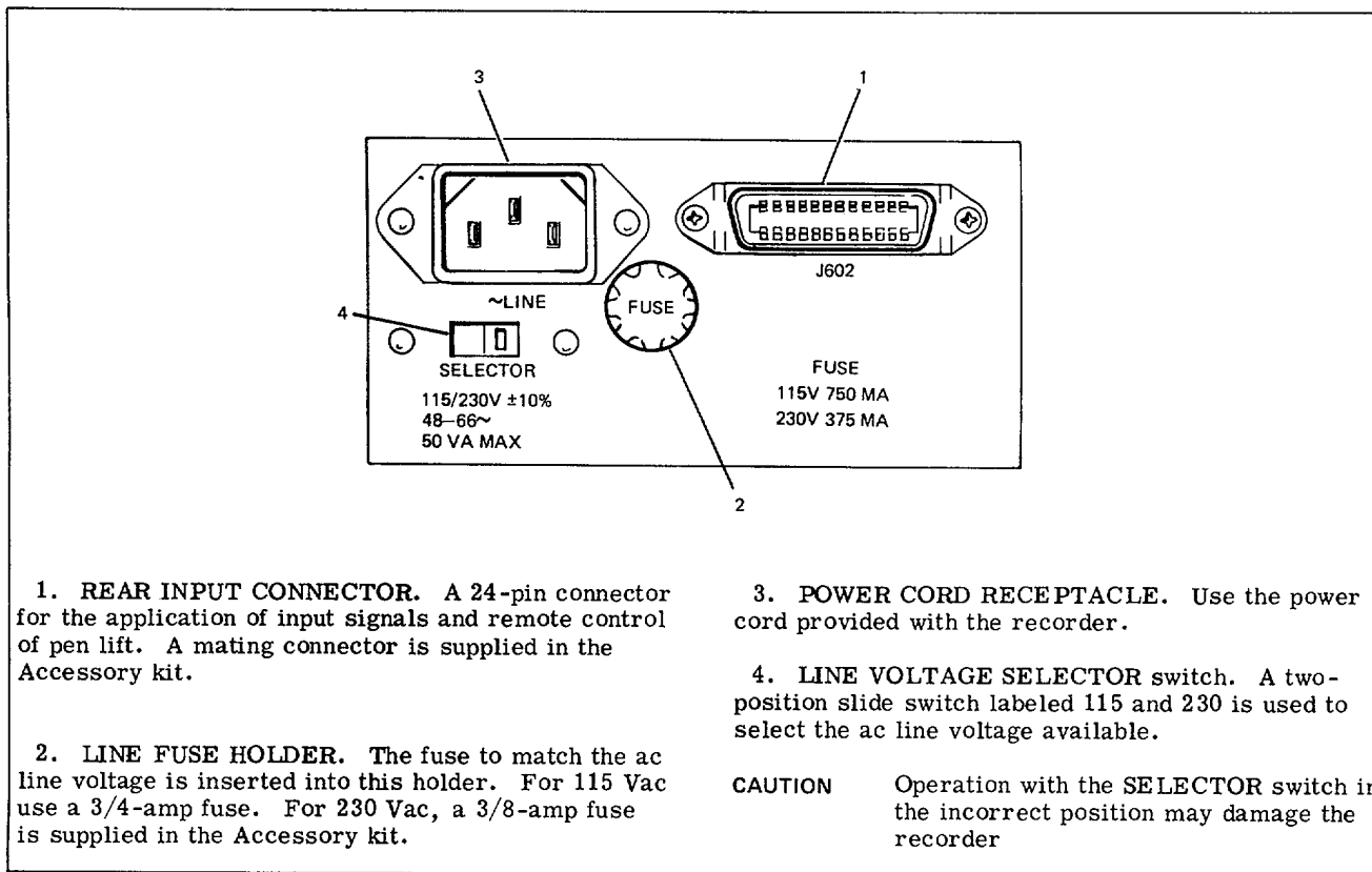
FIGURE 3-2. REAR PANEL
