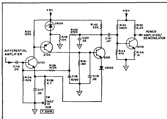
FIGURE 4-9. VOLTAGE AMPLIFIER
